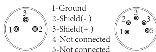
DMX-input XLR mounting-plugs
